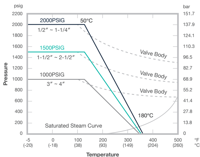
1/2" ~ 4" Reduced port Seat material : PTFE / RTFE
