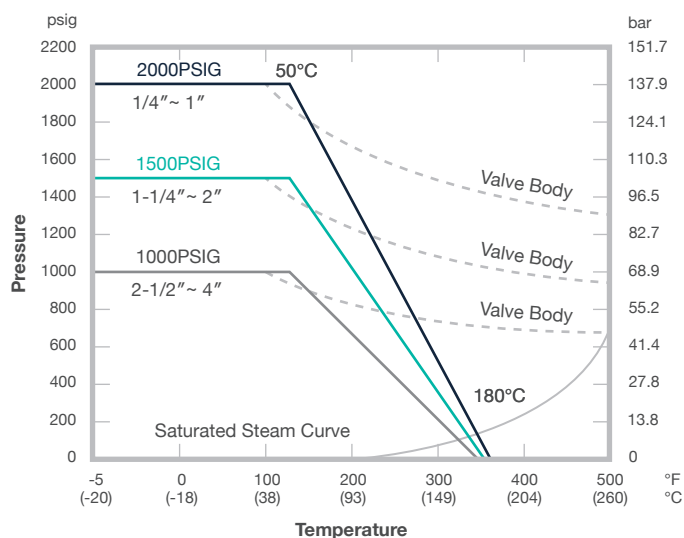
1/4" ~ 4" Full port Seat material : PTFE / RTFE
